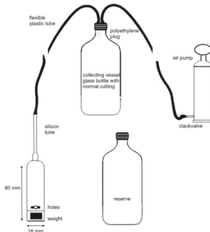
FIGURE 7.9.3 SIMPLE EQUIPMENT FOR GROUNDWATER SAMPLING.
