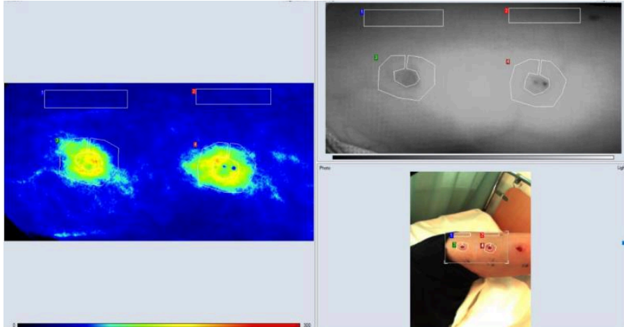
Figure 7. Blood perfusion analysis. Blood perfusion of wound edges was measured using LASCA (Laser Speckle Contrast Analysis) at MAD visits and analysed off-site as the difference in blood perfusion between the wound edge (drawn areas surrounding wounds marked green and dark red) and reference areas (top boxes, blue and red region) in each individual.
