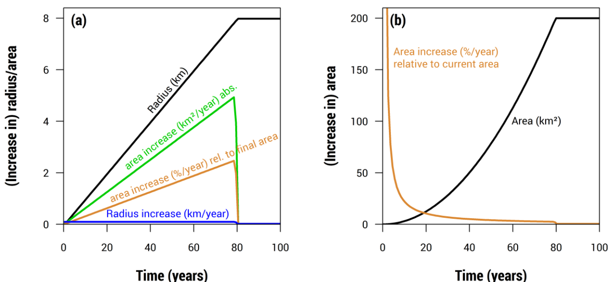
Figure II-2: Example of how different measures of expansion and expansion speed change over time. The figure is based on the assumption of a constant expansion potential, and the maximum colonisable area is set to 200 km 2 . Radius change (blue) is constant. The radius (black, panel a), the absolute area change (green) and the area change relative to the final area (orange, panel a) increase linearly with time. The area (black, panel b) increases quadratically with time. Area change relative to the current area (orange, panel b) decreases hyperbolically with time.
