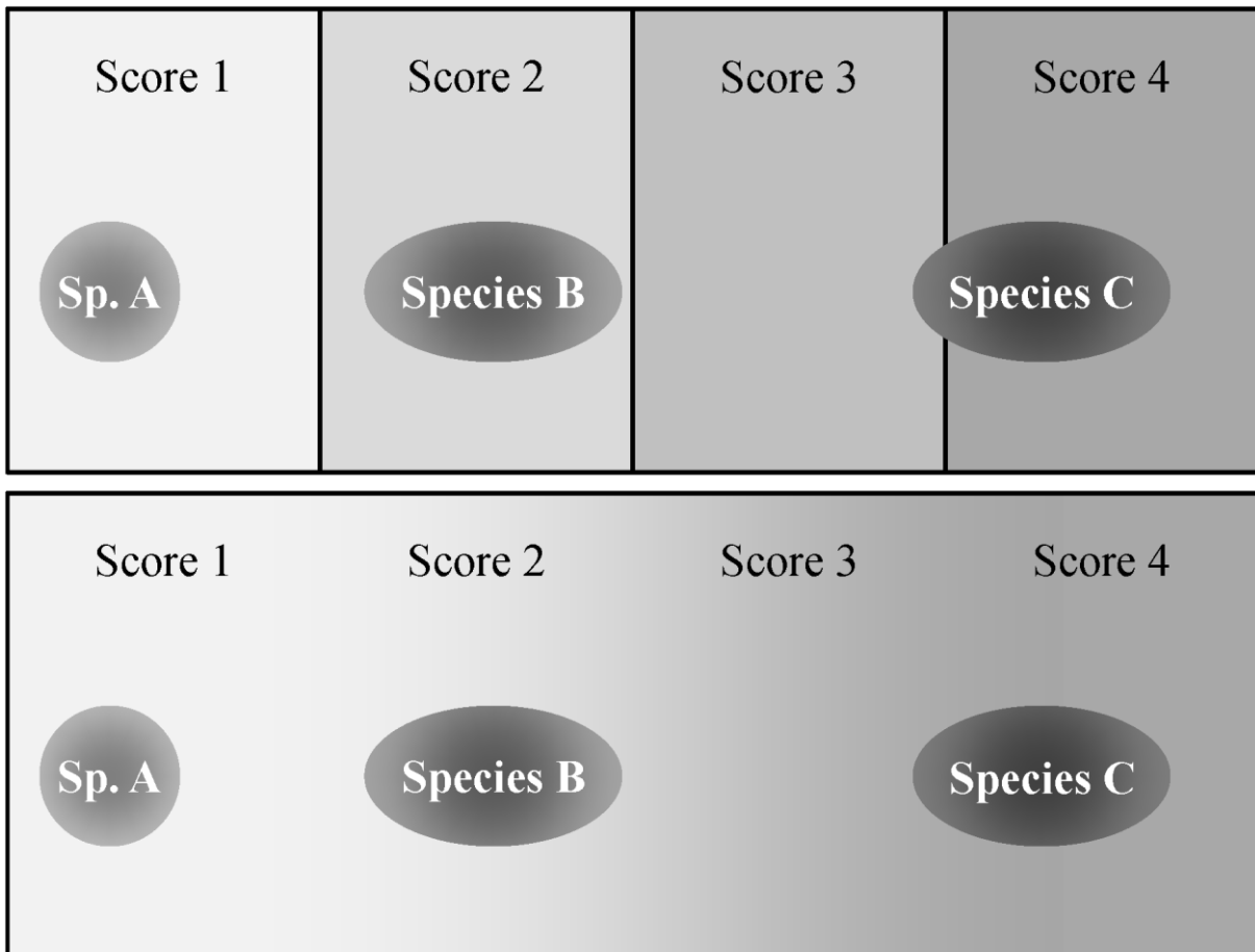
Figure III-1: Concept figure illustrating three species in an (a) quantitative and a (b) qualitative set of criteria.
