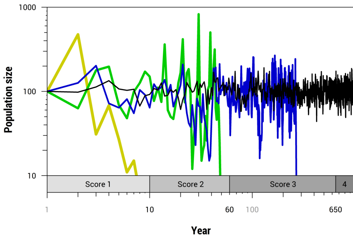
Figure 7: Illustration of criterion A. Example trajectories of population size over time, and time periods used as threshold values for population lifetime. The yellow/green/blue species have a lifetime of < 10/60/650 years, respectively; the black species of > 650 years. The significance of fluctuations is apparent from the figure: the larger the amplitude of the fluctuations (i.e., the larger the environmental variance), the shorter is the lifetime of the species. The four species have identical population growth rates ( \lambda = 1.6 ), carrying capacity ( K = 100 ) and demographic variance ( \sigma_d^2 = 0.1 ), but different environmental variance ( \sigma_e^2 = 1.2, 0.8, 0.5, 0.2 , respectively). NB: Both axes are on the log-scale.
