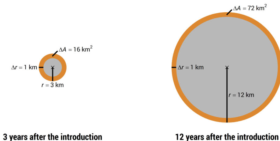
Figure II-1: Illustration of the same expansion process at two different time steps. The grey area is already colonised, the orange area is newly colonised in a given year. Assuming a constant expansion (i.e., assuming a constant radius change \Delta r per year), the change in area ( \Delta A per year) will itself increase over time.
