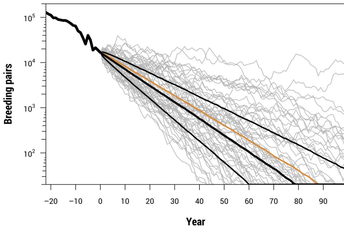
Figure 8: Example of a population viability analysis. Observed population numbers up to 2010 (negative years) and simulated numbers thereafter (positive years). Thin grey lines show some examples of simulated future trajectories. The three black lines show the quartiles (lower, median, upper) of all simulated trajectories; the orange line shows the 60th percentile. Lifetime is equivalent to the number of years until quasi-extinction, i.e. until the population crosses the quasi-extinction threshold (which was here set to 20 breeding pairs). The population is estimated to go extinct within 60 to 112 years (lower/upper quartile), with a median lifetime of 79 years and a 60th percentile of 88 years. Please note that the y-axis is on the logarithmic scale. The example is one population of Rissa tridactyla . (Source: Sandvik et al. 2014, modified)
