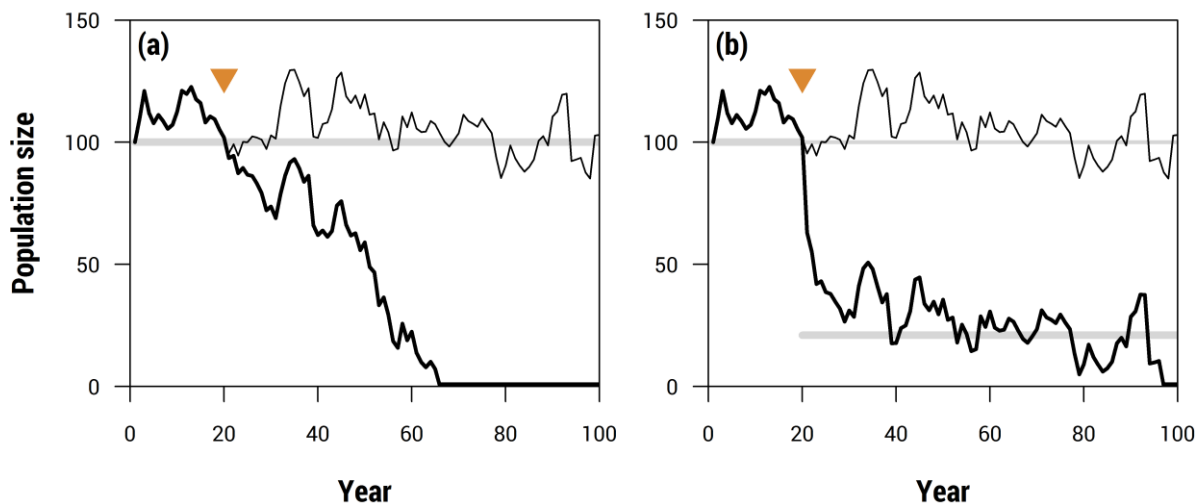
Figure 3: Illustration of population growth rate and carrying capacity. The curves show the population dynamics of a population. The thin line indicates the population trajectory in the absence of disturbance (e.g., by an alien species). The thick line indicates the population trajectory when (a) the population growth rate is reduced and (b) the carrying capacity is reduced. The change in growth rate / carrying capacity occurs at the time marked by the orange arrowhead. The horizontal grey lines indicate the respective populations' carrying capacities. A negative growth rate will inevitably lead to extinction; a reduced carrying capacity will do so only if the population fluctuations (or the environmental variance) are sufficiently large.
