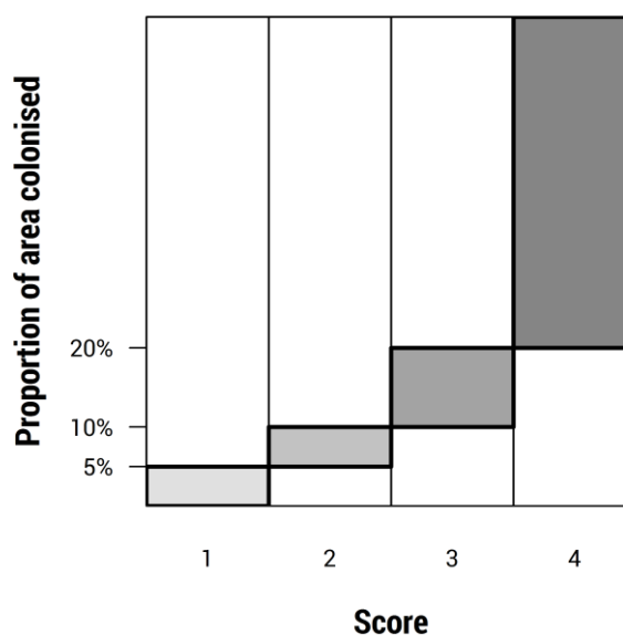
Figure 5: Illustration of criterion C. The score according to this criterion is based on the proportion of the area of a nature type colonised by the alien species.
