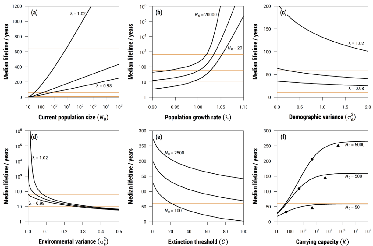
Figure X-1: Sensitivity of lifetime for the different parameters. Orange lines mark the threshold values of criterion A. (a) Median lifetime increases with increasing population size ( N_0 ). Shown for three different population growth rates ( \lambda = 0.98, 1.00, 1.02 ; other parameters: \sigma_d^2 = 0.5, \sigma_e^2 = 0.05, C = 10, K = 100 \cdot N_0 ). Note that the x-axis is on log-scale. (b) Median lifetime increases with increasing population growth rate ( \lambda ). Shown for three different population sizes ( N_0 = 20, 100, 20\,000 ; other parameters: \sigma_d^2 = 0.5, \sigma_e^2 = 0.05, C = 10, K = 100 \cdot N_0 ). Note that the y-axis is on log-scale. (c) Median lifetime decreases with increasing demographic variance ( \sigma_d^2 ). Shown for three different population growth rates ( \lambda = 0.98, 1.00, 1.02 ; other parameters: N_0 = 100, \sigma_e^2 = 0.05, C = 10, K = 10\,000 ). (d) Median lifetime decreases with increasing environmental variance ( \sigma_e^2 ). Shown for three different growth rates ( \lambda = 0.98, 1.00, 1.02 ; other parameters: N_0 = 100, \sigma_d^2 = 0.5, C = 10, K = 10\,000 ). Note that the y-axis is on log-scale. (e) Median lifetime decreases with increasing quasi-extinction threshold ( C ). Shown for three different population sizes ( N_0 = 100, 500, 2500 ; other parameters: \lambda = 1.01, \sigma_d^2 = 0.5, \sigma_e^2 = 0.05, C = 10, K = 100 \cdot N_0 ). (f) Median lifetime increases with increasing carrying capacity ( K ). Shown for three different population sizes ( N_0 = 50, 500, 5000 ; other parameters: \lambda = 1.01, \sigma_d^2 = 0.5, \sigma_e^2 = 0.05, C = 10 ). If carrying capacity can be assumed to be at least 100 times population size (arrow heads), its precise value is of negligible significance. The dots mark situations where K = N_0 . Note that the y-axis is on logarithmic scale.
