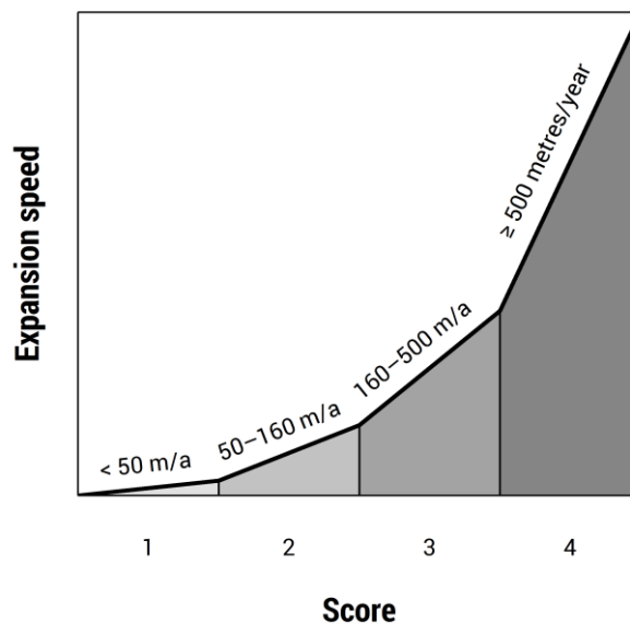
Figure 9: Illustration of criterion B. Expansion speed, defined as the annual rate at which the area of occupancy increases, is the basis for the score due to this criterion.
