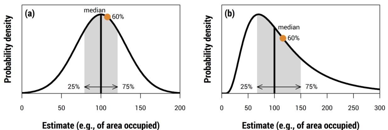
Figure 4: Examples of probability distributions. Estimates of empirical quantities follow a probability distribution, here exemplified by (a) a symmetrical (normal distribution) and (b) an asymmetrical (log-normal) distribution. The vertical line shows the median (entailing that it is equally likely that the true value is above and below this value). The grey area emphasises the interquartile range (or 50% confidence interval), i.e. the interval that contains the true value with a likelihood of 50%. The interquartile range is enclosed by the 25th percentile (lower quartile) and the 75th percentile (upper quartile). The 60th percentile is marked by the orange dot.
