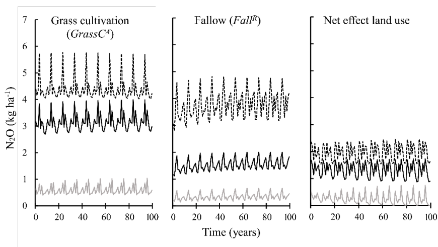
Figure 17. Annual nitrous oxide ( \text{N}_2\text{O} ) emissions from soil in (left) the grass system and (centre) from fallow land, and (right) net emissions from biogas feedstock cultivation during 100 years for all sites ( N=1240 ). The dashed black line represents the 95th percentile soil (max), the grey line the 5th percentile soil (min) and the black line the median soil.
