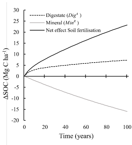
Figure 6. Cumulative change in soil organic carbon (SOC) over 100 years, simulated with DNDC model, for winter wheat cultivation with biogas digestate as fertiliser (dashed), mineral fertiliser (grey) and the net effect, i.e. the difference between digestate and mineral fertiliser (black). The DNDC model was executed with the input parameters setup that represented the average conditions in the region.
