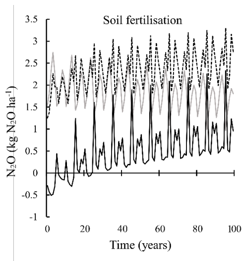
Figure 18. Annual nitrous oxide ( \text{N}_2\text{O} ) emissions from soil over a 100-year time horizon following fertilisation of winter wheat. The grey line represents emissions from winter wheat cultivation with mineral fertiliser, the black dashed line emissions from winter wheat cultivation with digestate. The black line shows the net effect, i.e. the difference between digestate and mineral fertiliser.
