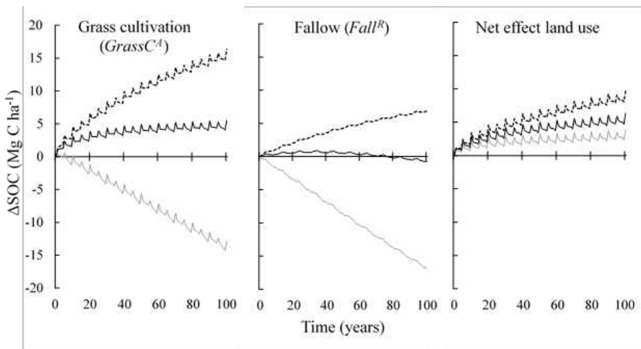
Figure 14. Simulated cumulative change in soil carbon (C) sequestration in the study region of Uppsala municipality. Change in C stock ( \text{Mg C ha}^{-1} ) for (left) grass cultivation only and (centre) fallow only, and (right) net effect of the land use, i.e. grass cultivation – fallow. The grey line represents the 5th percentile in the region, the black line the median and the dashed black line the 95th percentile.
