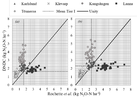
Figure 5. Cumulative yearly \text{N}_2\text{O} emissions ( \text{kg N}_2\text{O-N ha}^{-1} ) estimated with three different methods for fertilisation rate (a) F1 and (b) F2. The results obtained for the Rochette et al. approach are shown on the x-axis and those obtained with the DNDC model on the y-axis. The black line represents unity in the two site-dependent methods and the black dashed line represents mean emissions across all sites calculated with IPCC Tier 1.
