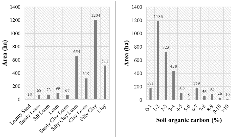
Figure 5. Soil texture and initial soil organic carbon (SOC) content at sites under fallow (N=1240) in Uppsala municipality used in Paper II.
