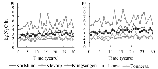
Figure 4. Cumulative yearly N 2 O emissions from the study sites (kg N 2 O ha -1 ), estimated using the DNDC model, for fertilisation rate (a) F1 and (b) F2 over the 30-year simulation period.
