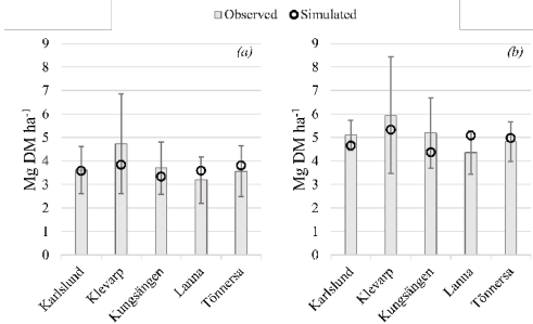
Figure 9. Aboveground mean biomass production at harvest, with fertilisation rate F1 (a) and F2 (b). Bars represent mean of the observations, the rings simulated means and the error bars the standard deviation of the observations.
