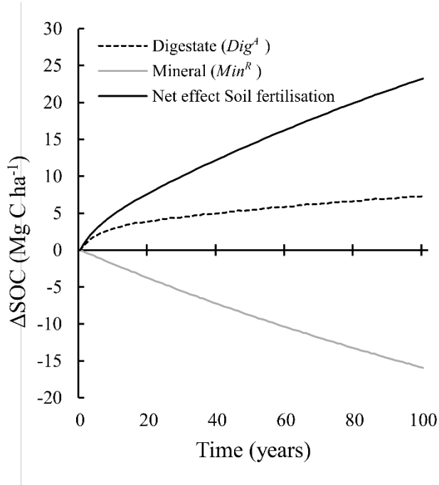
Figure 16. Simulated soil carbon (C) sequestration in winter wheat cultivation using mineral fertiliser (grey), digestate fertiliser (dashed) and the net effect, i.e. digestate – mineral. Modelled for one field, which represented average conditions in the study region
